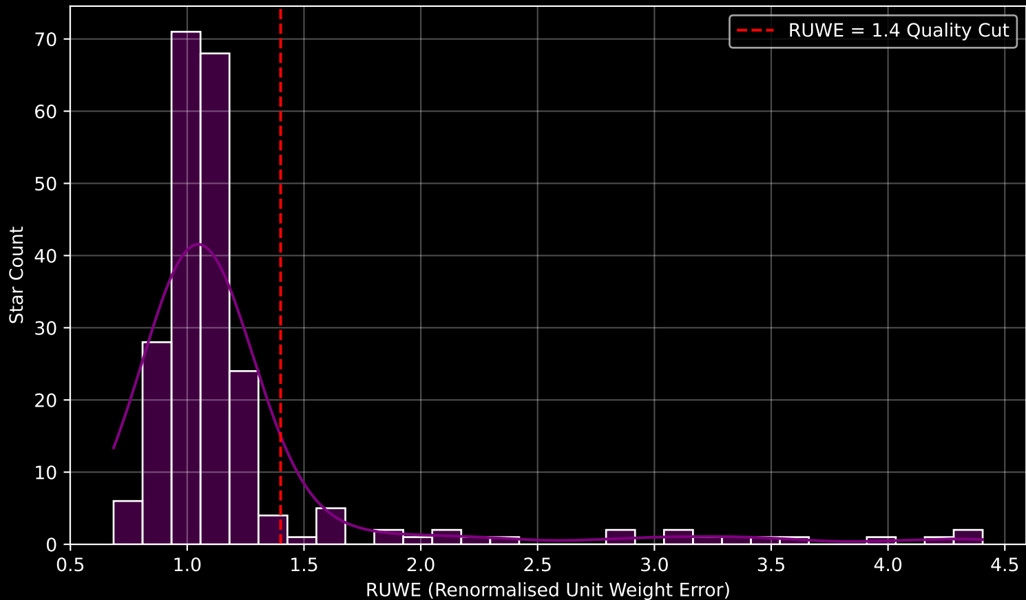
GALAH DR4 Field [7192] RUWE Distribution (n= 226)
