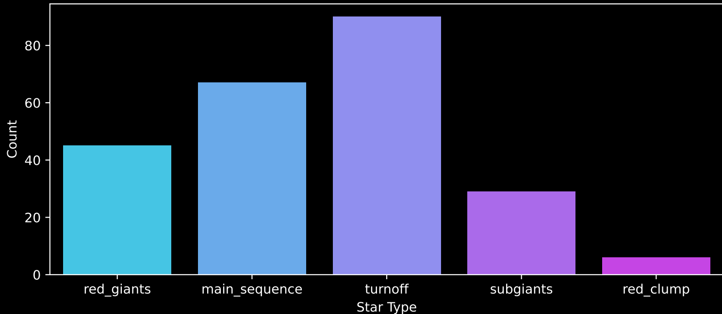
GALAH DR4 Field: [7192] Count plot of Star Type
