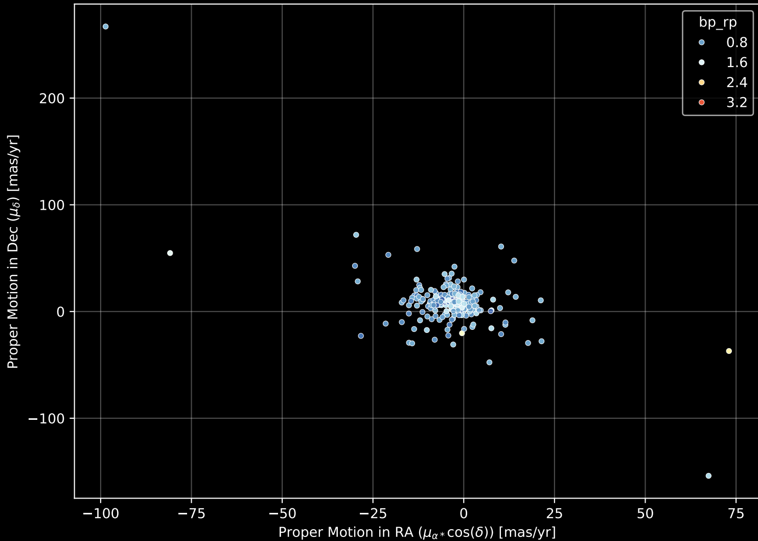
GALAH DR4 Field: [7192] Proper Motion Diagram (n= 237)
