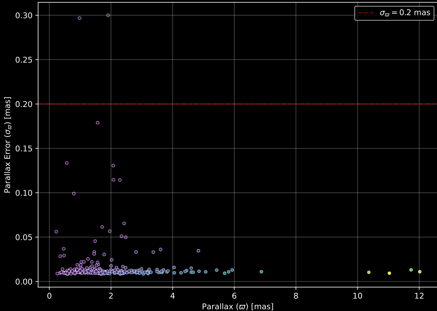
GALAH DR4 Field: [7192] Parallax Quality (n= 237)
