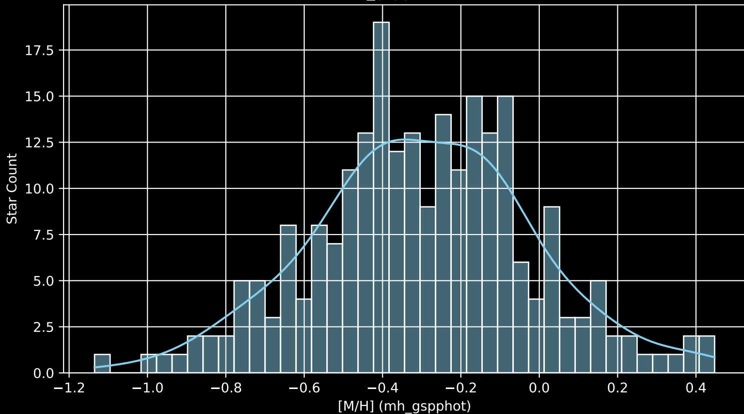
GALAH DR4 Field: [7192] [M/H] (mh_gspphot) (n= 236)
