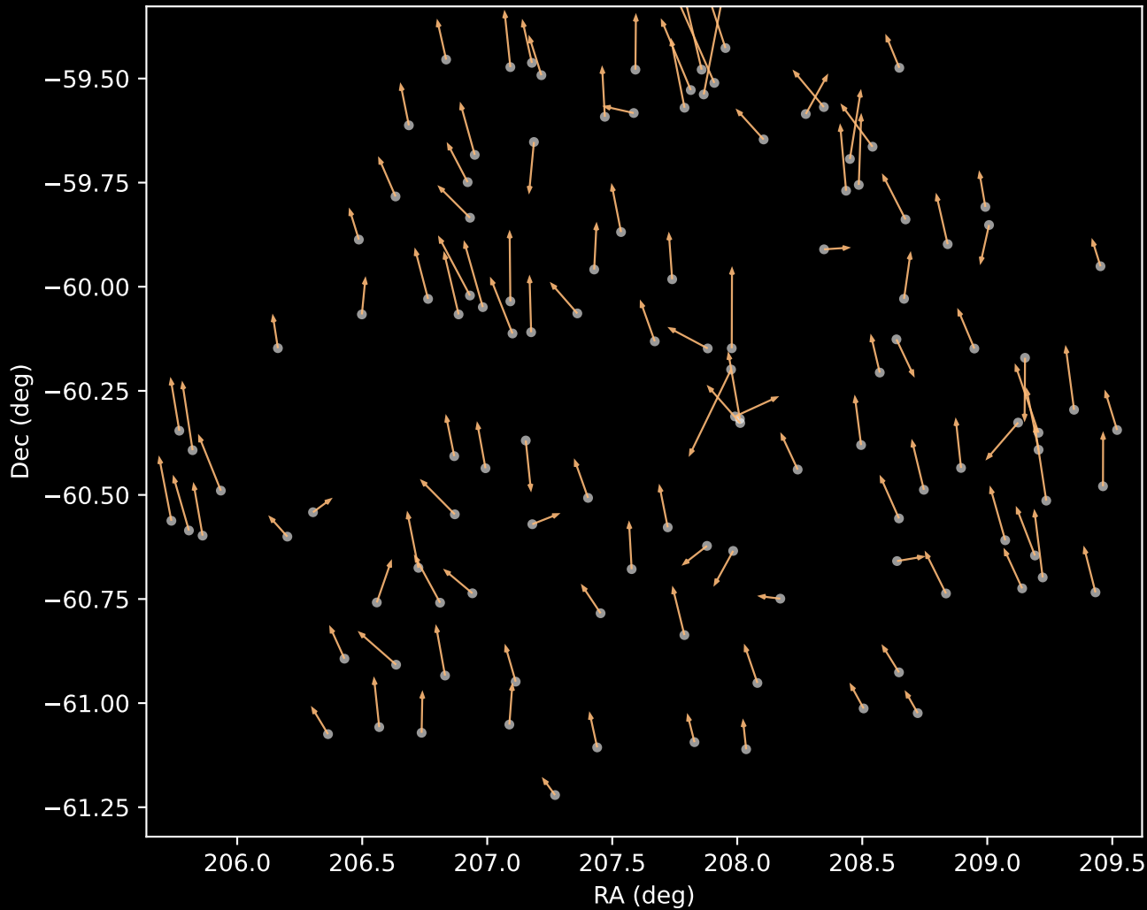
GALAH DR4 Cluster 3 Proper Motion Vectors (n=119)
